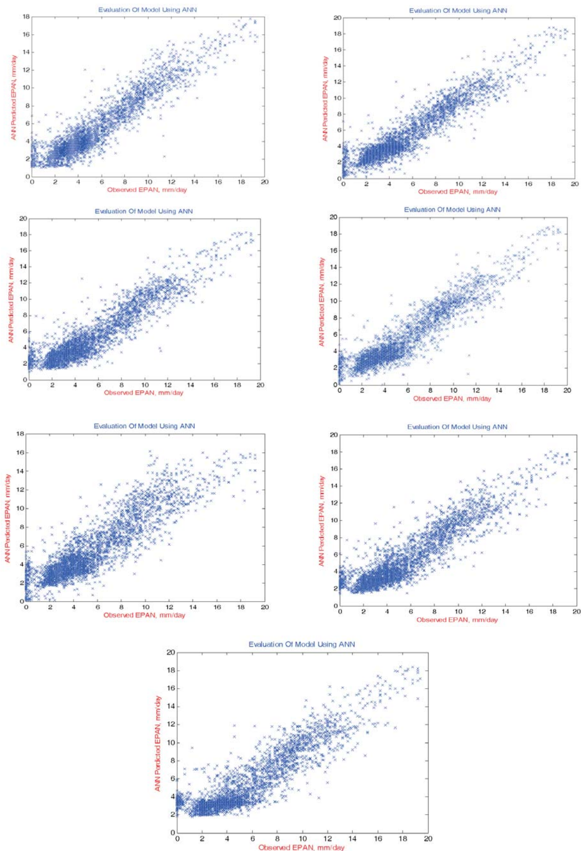
Fig. 2. Observed and predicted EPAN with General models (GM M1- M7) development data
