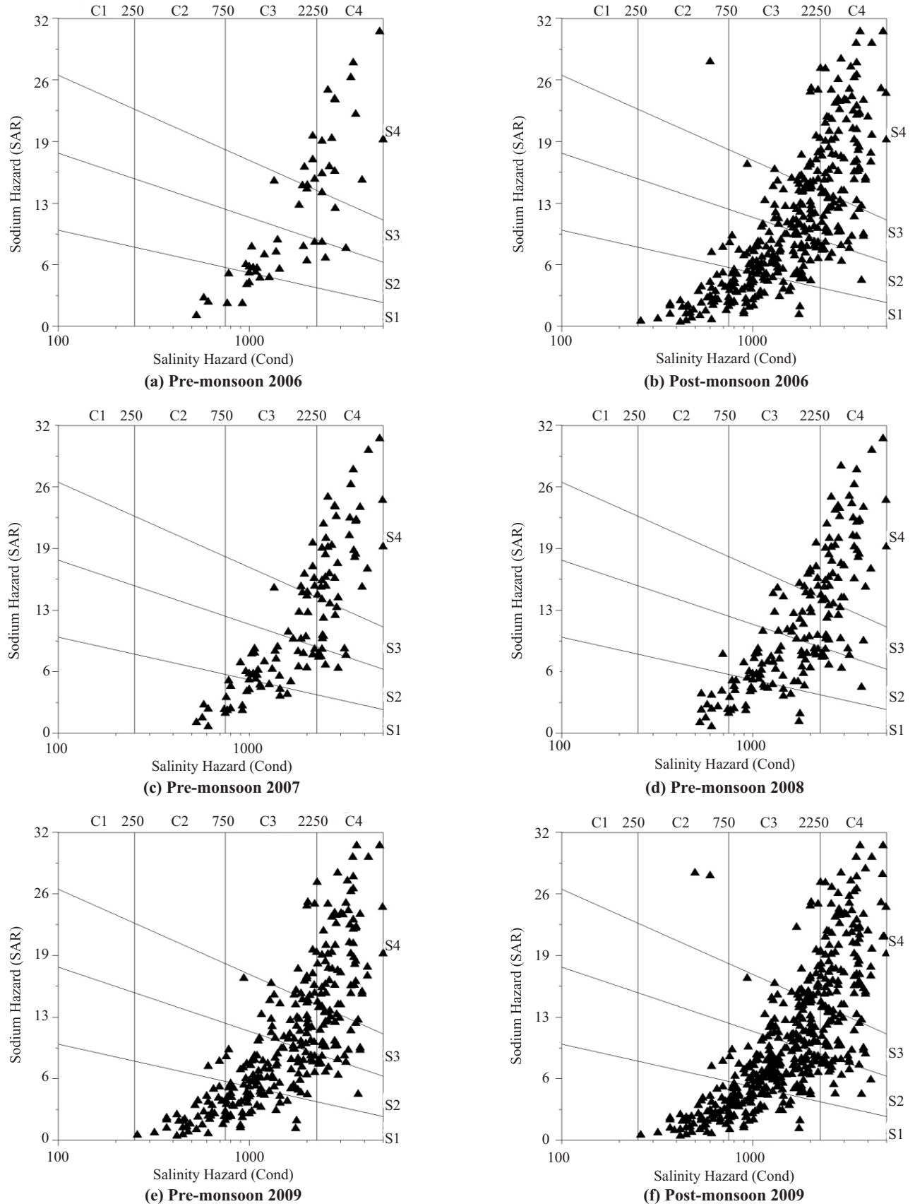
Fig. 3. USSSL diagrams showing suitability of groundwater for irrigation (Sodium hazard: S 1 - Low, S 2 - Medium, S 3 -High, S 4 - Very High; Salinity Hazard: C 1 - Low, C 2 - Medium, C 3 - High, C 4 - Very High)
