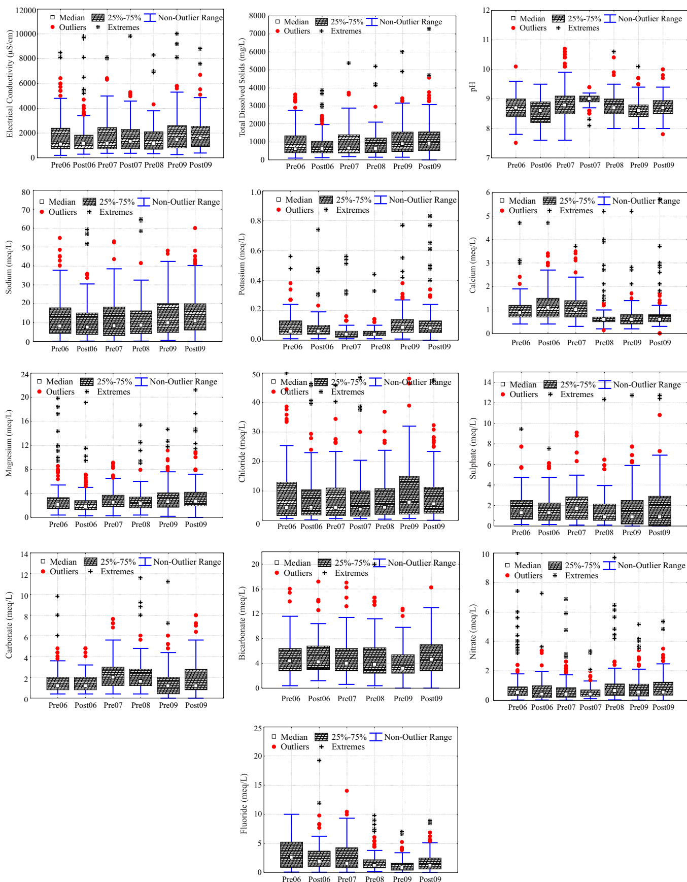
Fig. 2. Box and whisker plots of 13 groundwater quality parameters
