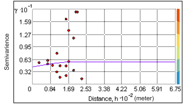
Fig. 2a. Semi variance and fitted models for pre monsoon ground water salinity in 2013
