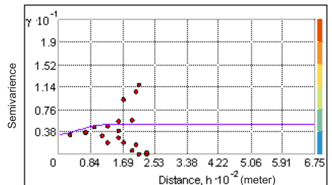
Fig. 2c. Semi variance and fitted models for pre monsoon ground water salinity in 2015
