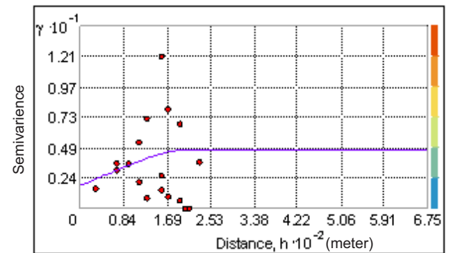
Fig. 2b. Semi variance and fitted models for post monsoon ground water salinity in 2013
