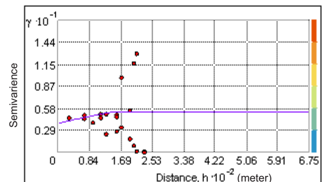
Fig. 2d. Semi variance and fitted models for post monsoon ground water salinity in 2015
