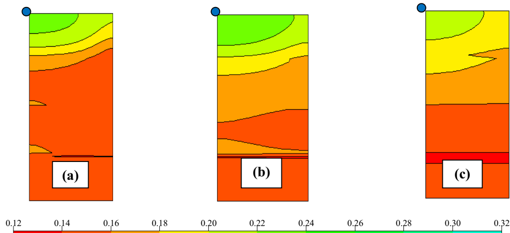
Fig. 6. Simulated water distribution (%) after a) 24 b) 48 and c) 72 h of fertigation
