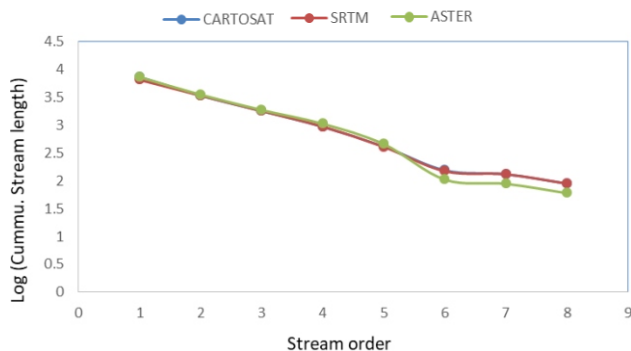
Fig. 4. Relationship between stream order and cumulative stream length
